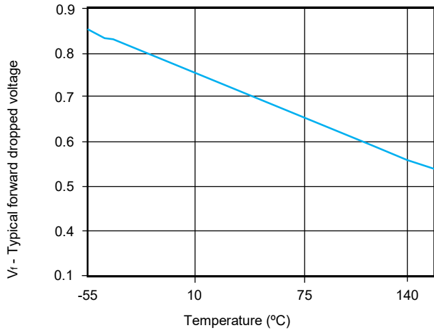
FIGURE 5 Forward Voltage
